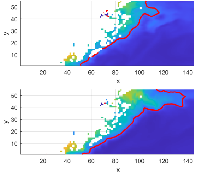
Fig. 2. CMEMS simulation data of chlorophyll a in the Baltic Sea, at two different time instances hours apart, with higher concentration (yellow), lower concentration (blue), land (white), and the front F(t) (red line).
