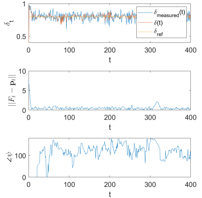
Fig. 7. First plot: difference between the noisy measured chlorophyll a concentration \delta_{\text{measured}}(t) , local chlorophyll a concentration \delta(t) , and the reference chlorophyll a concentration \delta_{\text{ref}} . Second plot: distance from the USV to the closest point in the front, \|F(t) - \mathbf{p}(t)\| . Third plot: angle of the estimated gradient, \angle\psi(t) .
