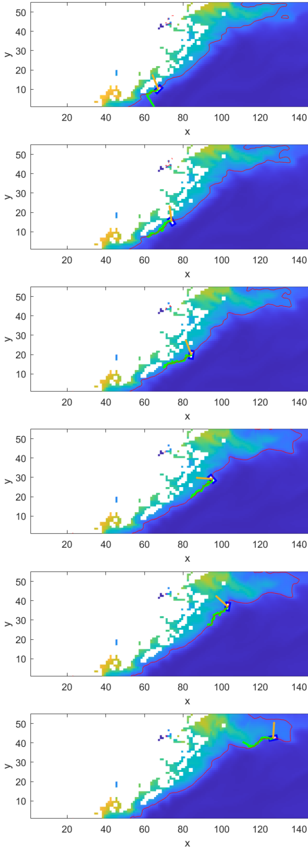
Fig. 6. Time-lapse of the USV (blue rectangle) and its gradient estimator \hat{\psi} (red arrow) tracking the algal front (indicated with red contour lines) with representation of USV's path (green).
